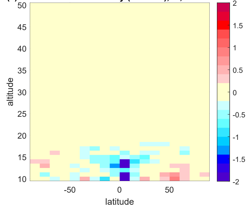
(f) Difference in uncertainty (old-new), %, 2015-2020
