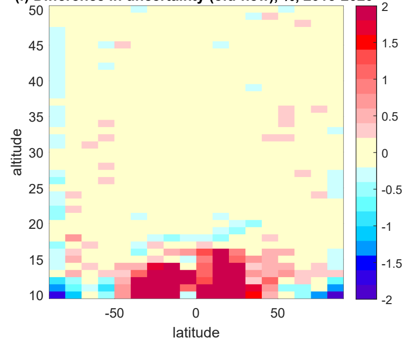
(f) Difference in uncertainty (old-new), %, 2015-2020
