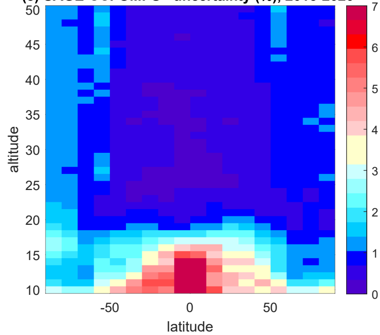
(e) SAGE-CCI-OMPS+ uncertainty (%), 2015-2020
