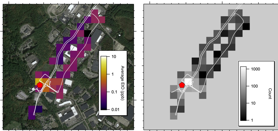
Figure S13. Binned average EtO concentrations downwind of Facility B (left) along with data point count (right). The facility is located at the red marker. Wind was from the West during these measurements. Map underlay: Google, © 2022 CNES / Airbus, MassGIS, Commonwealth of Massachusetts EOE, Maxar Technologies, RIGIS, USDA/FPAC/GEO
