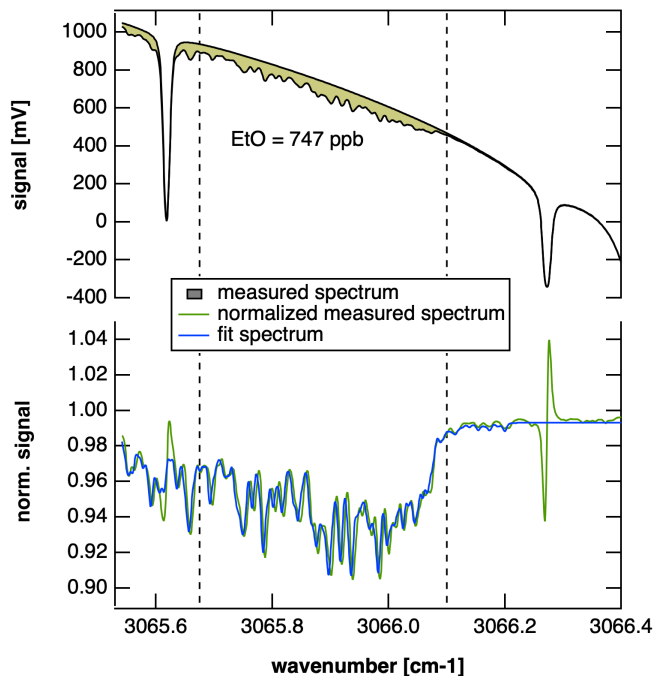
160 Figure S10. Summary spectra comparing instantaneous Facility A measurement of 747 ppb (in-plume, gold) to an out-of plume spectrum. The top shows signal as a function of wavenumber, with EtO contributions highlighted in yellow. The bottom shows a divided spectra in-plume/out-of-plume (green) and transmission simulation of EtO only.
