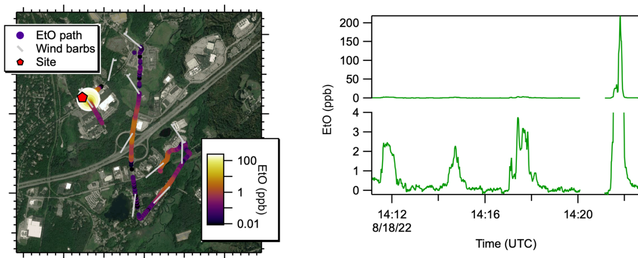
Figure S8. Detail of Morning Transect Downwind of Facility A. A map (left) shows AML path colored by EtO concentration (log scale), with wind barbs tethered to the truck path, and feather end of the staff pointing into the wind. Time series show EtO concentrations zoomed to 0-4 ppb (bottom right) and at full scale (top right). Map underlay: Google, © 2022 CNES / Airbus, Landsat / Copernicus, MassGIS, Commonwealth of Massachusetts EOEA, Maxar Technologies, USDA/FPAC/GEO
