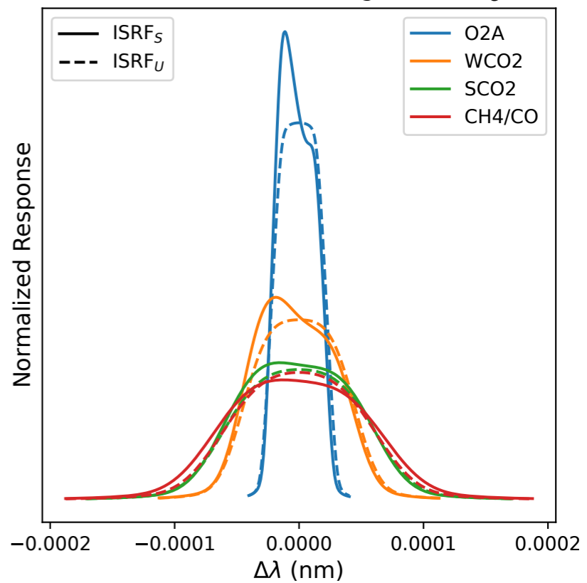
(c) MODIS Derived \text{ISRF}_S vs. \text{ISRF}_U
