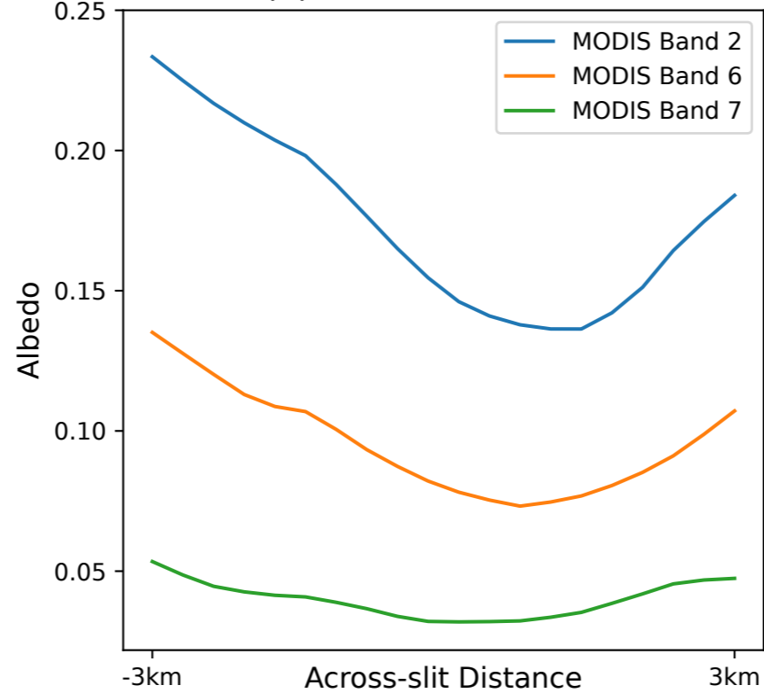
(b) MODIS Subslit Albedo
