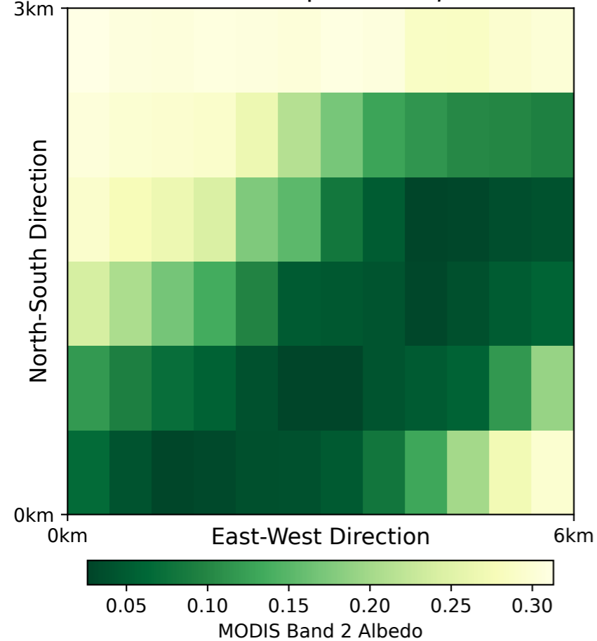
(a) GeoCarb Sub-Footprint 0.85\ \mu\text{m} Albedo
