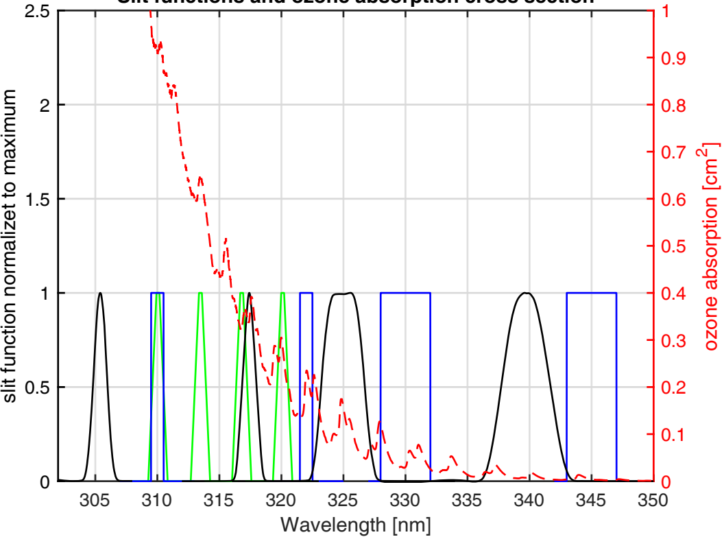
Slit functions and ozone absorption cross section
