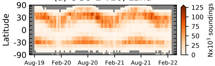
(a) OCO-2 v10, Land
