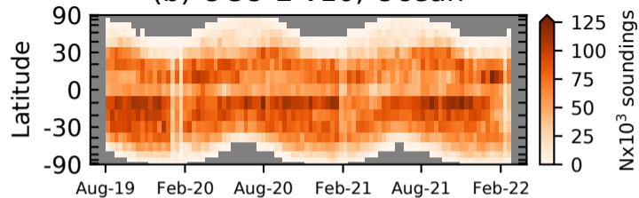
(b) OCO-2 v10, Ocean
