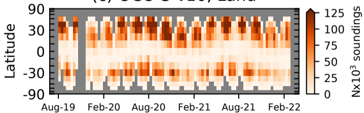
(c) OCO-3 v10, Land
