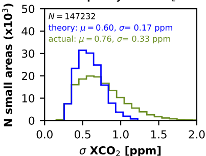
(c) OCO-3 v10, land-nadir frequency of \sigma XCO 2
