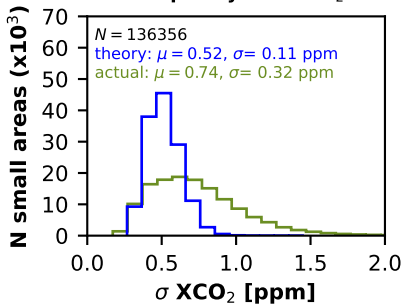
(a) OCO-2 v10, land-nadir frequency of \sigma XCO 2
