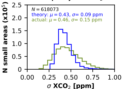
(a) OCO-2 v10, ocean-glint frequency of \sigma XCO 2
