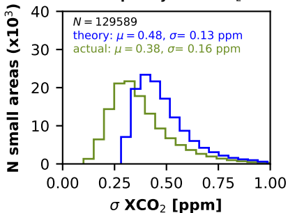
(c) OCO-3 v10, ocean-glint frequency of \sigma XCO 2
