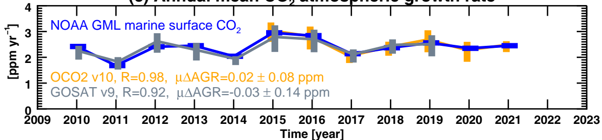
(c) Annual mean CO 2 atmospheric growth rate
