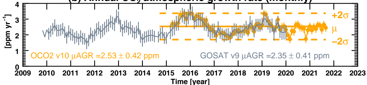
(b) Annual CO 2 atmospheric growth rate (monthly)
