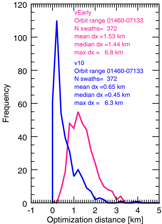
(a) OCO-3 SAM optimization distance Frequency
