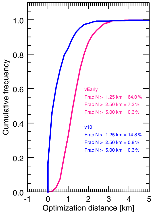
(b) OCO-3 optimization distance Cumulative Frequency
