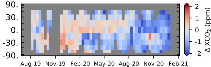
(a) OCO-3 v10 w/out adhoc, Land-Nadir
