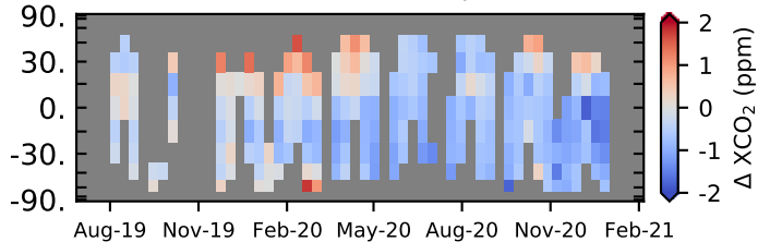
(b) OCO-3 v10 w/out adhoc, Ocean-Glint
