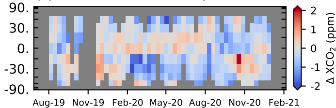
(c) OCO-3 v10 with adhoc, Land-Nadir
