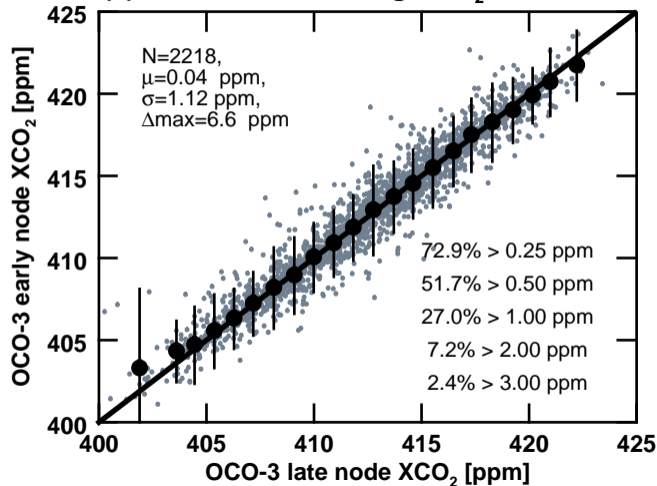
(a) OCO-3 self-crossing XCO 2 correlation
