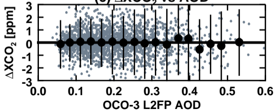
(c) \Delta\text{XCO}_2 vs AOD
