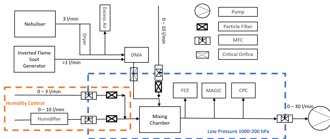
Figure 1. Flow schematic of the laboratory set-up for the low-pressure characterisation with two aerosol sources. The inline pressure is controlled via mass flow controllers (MFCs), the aerosol size classification is ensured with a differential mobility analyser (DMA), and the Faraday cup electrometer (FCE) functions as a reference instrument for particle counting.
