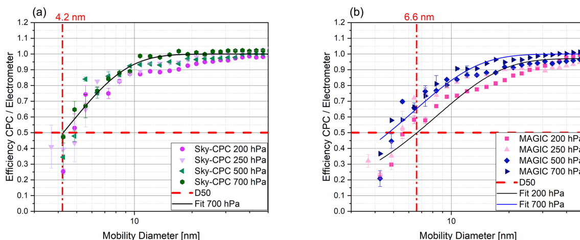
Figure 4. Compilation of the efficiency ratio curves of the SKY-CPC 5.411 (SKY-CPC) (a) and the MAGIC 210-LP CPC (b) to the FCE reference – at different operation pressures as a function of the particle size using ammonium sulfate particles. The variance of the measurement is indicated by vertical bars.
