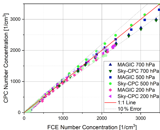
Figure 7. Comparison of the counting linearity between CPC and the electrometer at different pressure levels for fresh combustion soot.
