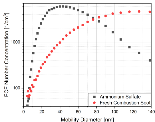
Figure 3. Particle size distributions were measured by an electrometer and sized by DMA for ammonium sulfate and fresh combustion soot. For this work, the particle mobility sizes were measured to 138 nm, so the size resolution at smaller sizes is suitable for the cut-off characterisation. The full particle size distributions are available (Weber et al., 2022).
