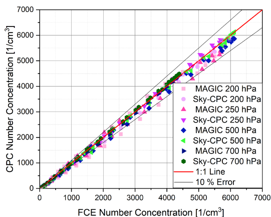
Figure 5. Comparison of the counting linearity between both CPC types and the electrometer at different pressure levels for nebulised ammonium sulfate.
