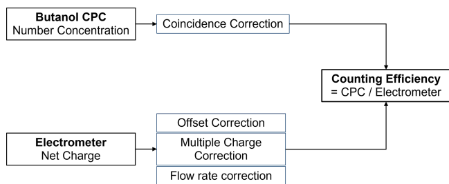
Figure 2. Flowchart of the data inversion procedure for particle concentration determination.
