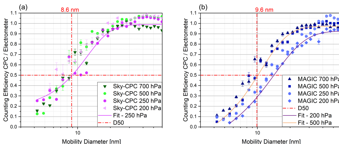
Figure 6. Comparison of the efficiency ratio curves of the SKY-CPC 5.411 (SKY-CPC) (a) and the MAGIC 210-LP CPC (b) to the electrometer reference at different operating pressures as a function of the particle size using fresh combustion soot. The variance of the measurement is indicated by vertical bars.
