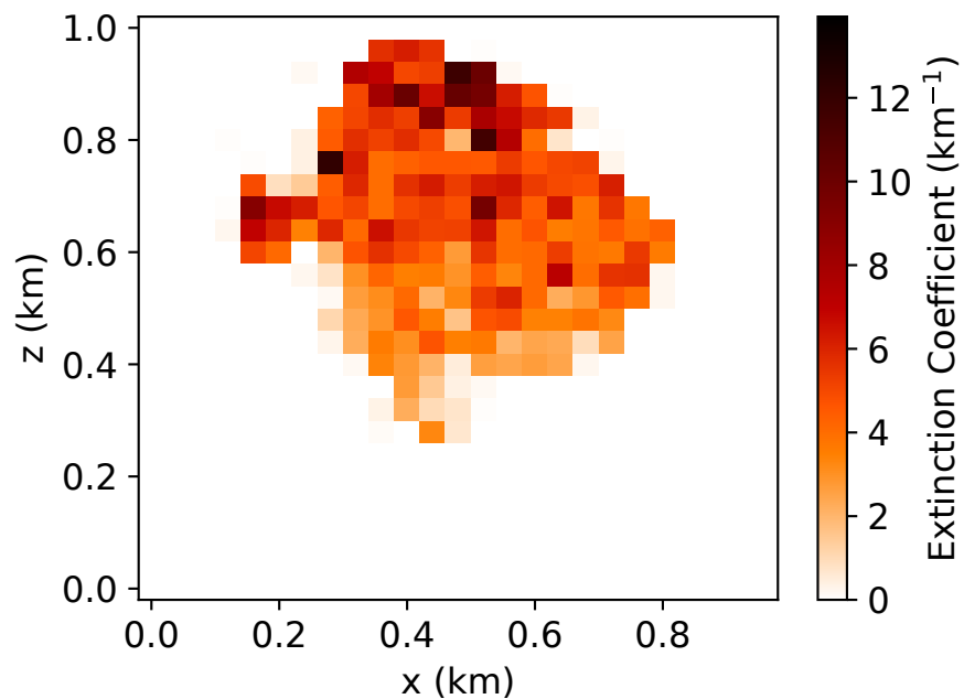
Retrieved Cross Section in Measurement Plane Default
