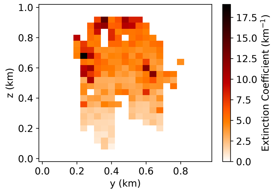
True Cross Section in Solar Plane
