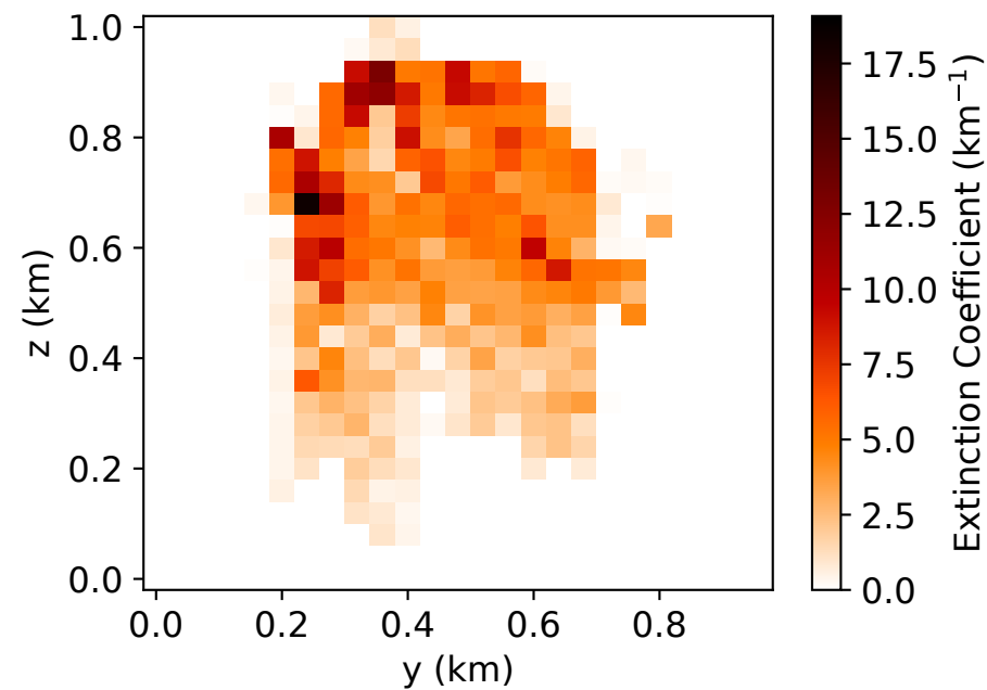
Retrieved Cross Section in Solar Plane Low
