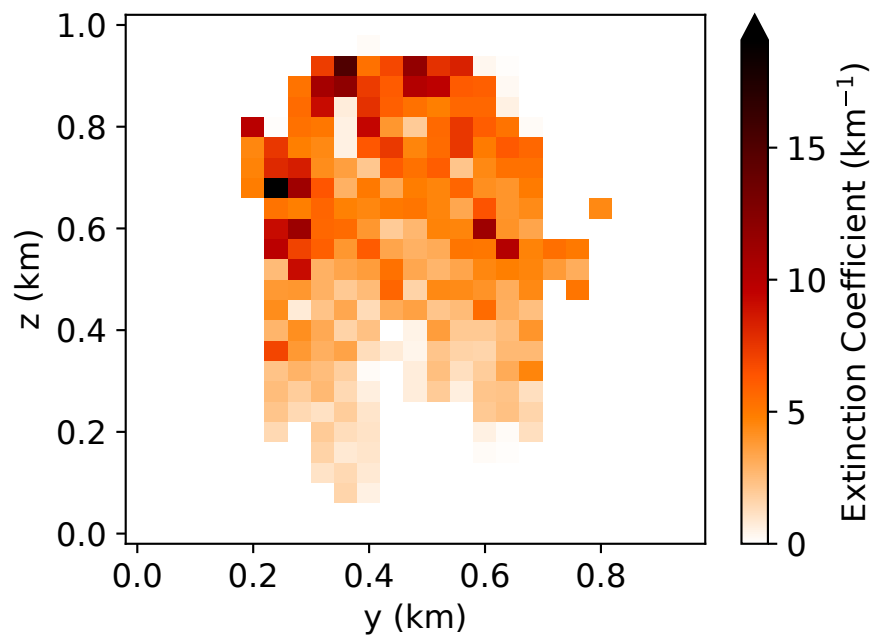
Retrieved Cross Section in Solar Plane Default
