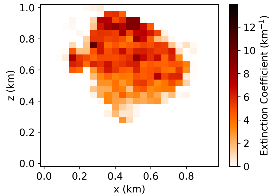
Retrieved Cross Section in Measurement Plane Low
