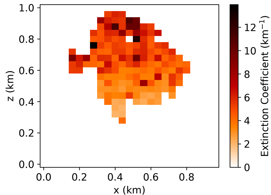
True Cross Section in Solar Plane
