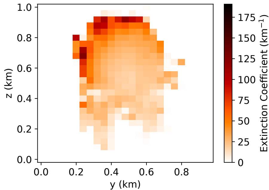
Retrieved Cross Section in Solar Plane Default
