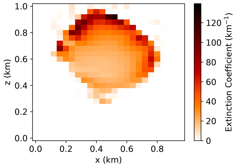
Retrieved Cross Section in Measurement Plane Default
