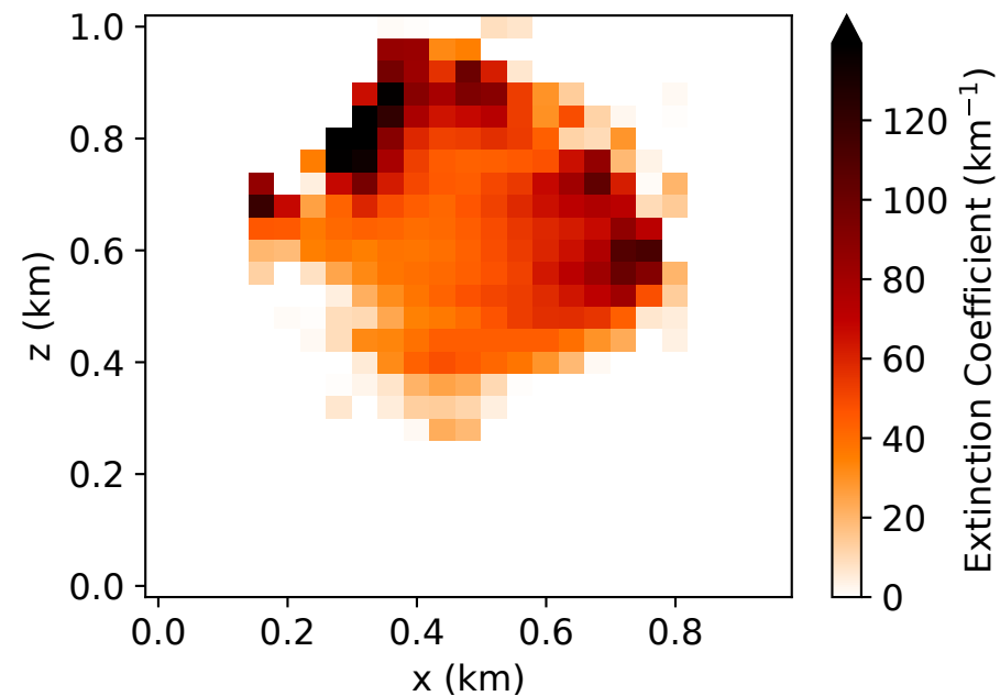
Retrieved Cross Section in Measurement Plane Low
