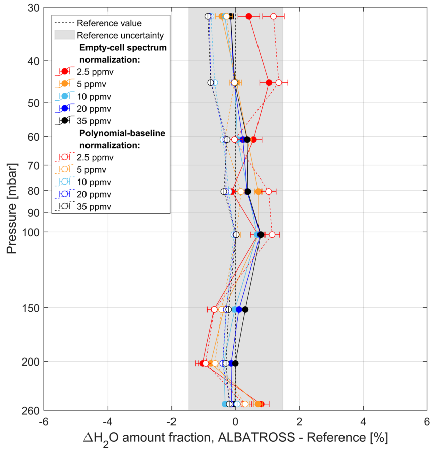
Figure S2. Comparison of accuracy assessed using the polynomial-baseline (open circles/dashed line) and the empty-cell spectrum (solid circles/solid line) normalization approaches. The relative differences in \text{H}_2\text{O} amount fraction ( \Delta\text{H}_2\text{O} ), between the ALBATROSS retrievals and the reference values are shown as function of pressure and \text{H}_2\text{O} amount fraction (color-coded as in Figure 8).
