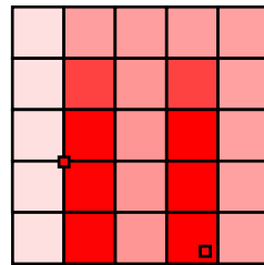
(c) ■ Dodecane
