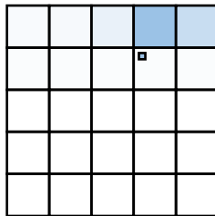
(e) ■ Adamantane
