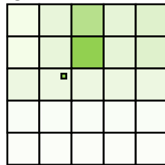
(g) ■ α-Pinene
