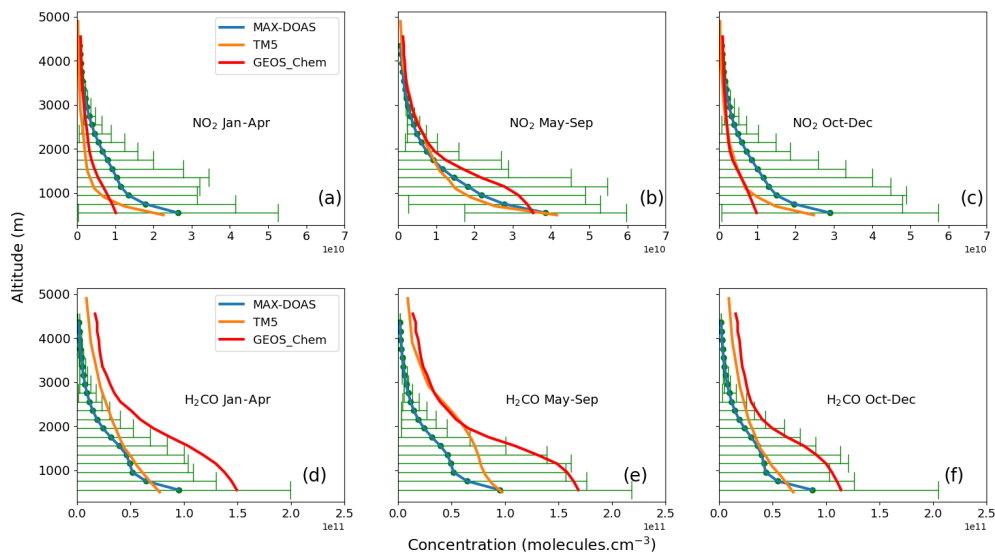
Figure C1. MAX-DOAS, TM5 and GEOS-Chem median profiles of \text{NO}_2 (a, b, c) and \text{H}_2\text{CO} (d, e, f). The error bars represent the standard deviation.
