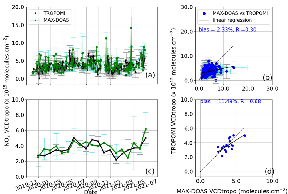
Figure 10. Case 2 – NO 2 : comparison of daily (a) and monthly (c) tropospheric vertical column densities of MAX-DOAS (green dots) and TROPOMI (black dots) over Kinshasa from 1 November 2019 to 1 July 2021. The MAX-DOAS is the hourly average coincidence day of TROPOMI satellite overpass. The individual TROPOMI points are those obtained from Eqs. (1) and (2) as described in the second case. Error bars are (1 \sigma ) standard deviations. (b, d) Least-squares linear regressions between the two datasets.
