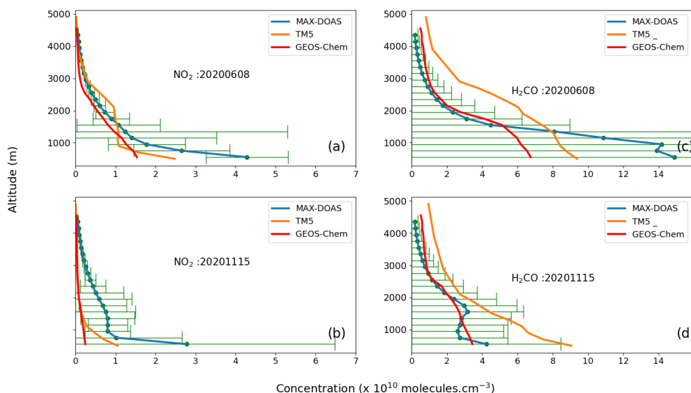
Figure 6. MAX-DOAS, TMS and GEOS-Chem median profiles of \text{NO}_2 (a, b) and \text{H}_2\text{CO} (c, d). The error bars represent the standard deviation. The daily MAX-DOAS median profiles shown in green dots are illustrated by the type of profile used to recalculate the tropospheric vertical column densities according to Eqs. (1) and (2).
