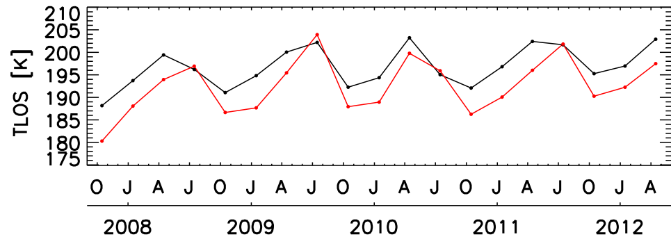
30–50°N 95 km
