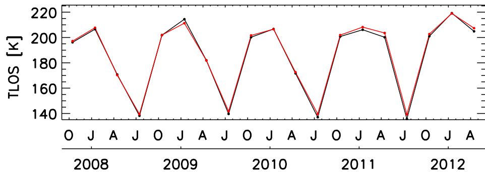
70–90°N 85 km
