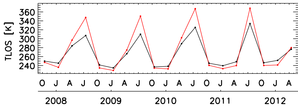
70–90°N 100 km
