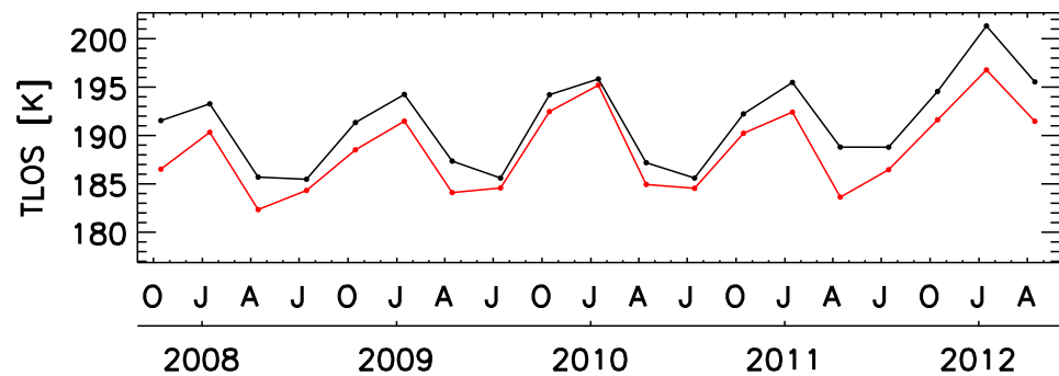
30–50°N 85 km
