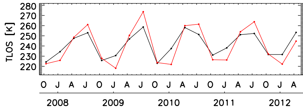
30–50°N 100 km
