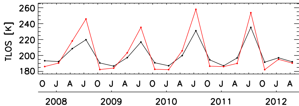
70–90°N 95 km
