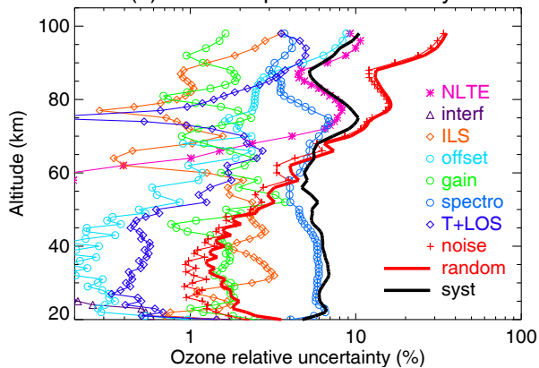
(e) Northern polar summer day MA
