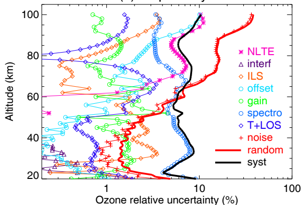
(c) Northern midlatitude spring day MA
