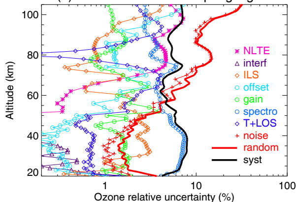
(f) Southern polar winter night MA
