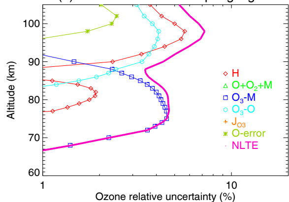
(f) Southern polar winter night MA
