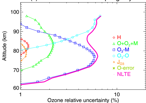
(e) Northern polar summer day MA
