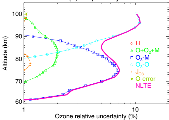
(c) Northern midlatitude spring day MA
