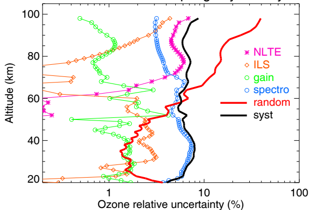
Northern polar summer day MA Syst
