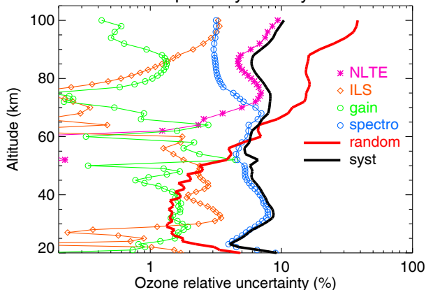
Northern midlatitude spring day MA Syst
