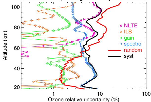
Northern midlatitude spring night MA Syst
