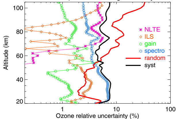
Southern polar winter night MA Syst
