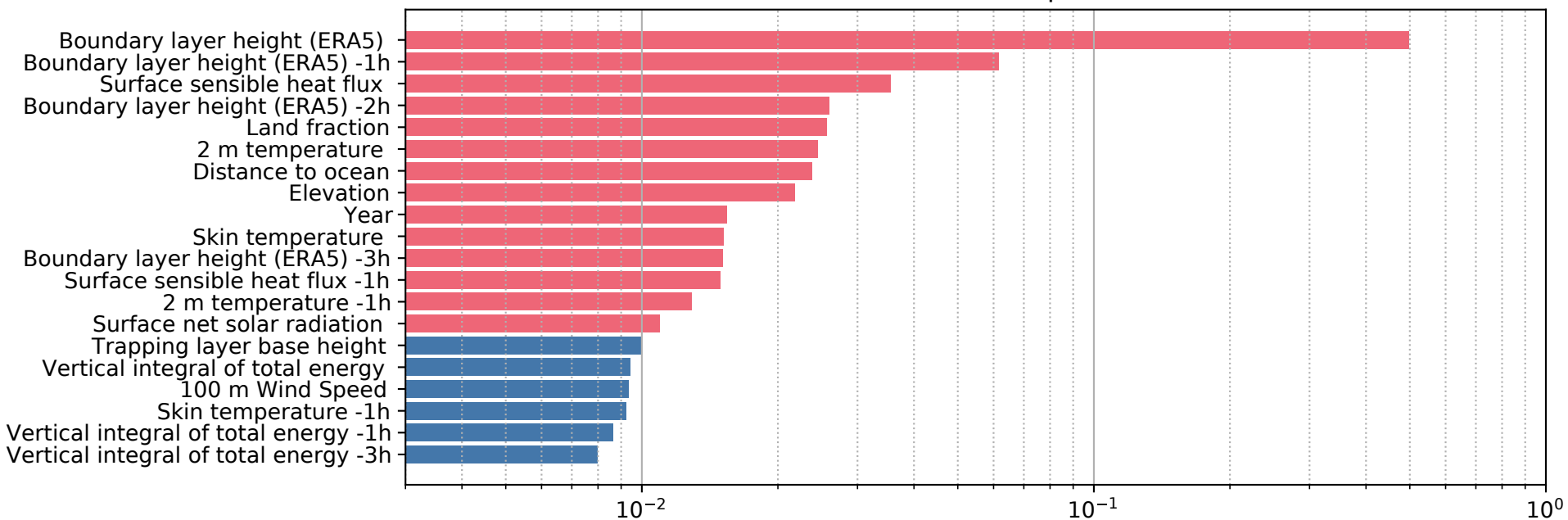
(b) SHAP feature importance
