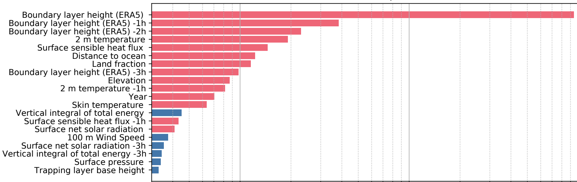
(b) SHAP feature importance
