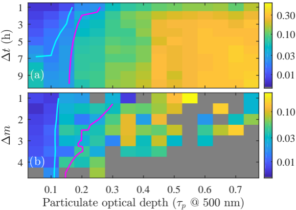
Temporal & spatial \sigma_\tau , contours at 0.014 & 0.028
