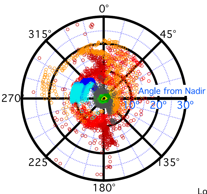
(a) End-of-Fiber Position
