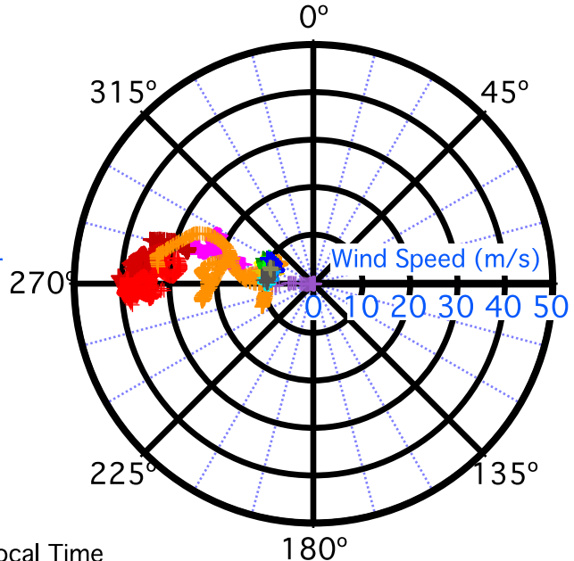
(b) Gondola-Level Winds
