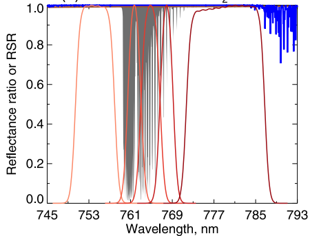
(b) OLCI RSRs near O 2 A-band
