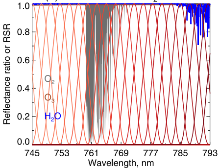
(a) OCI RSRs near O 2 A-band
