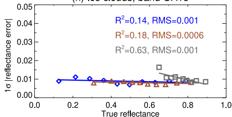
(h) Ice clouds, band OA15
