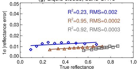
(g) Liquid clouds, band OA15
