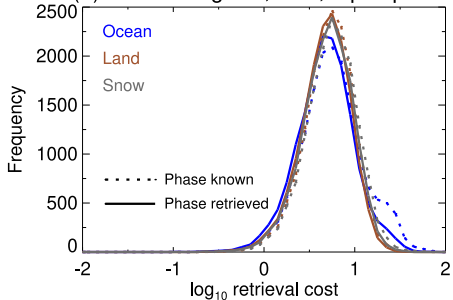
(a) Cost histogram, OCl, liquid phase
