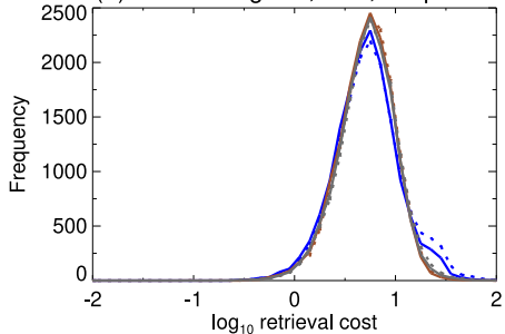
(b) Cost histogram, OCl, ice phase
