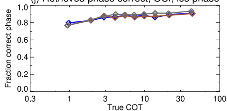
(j) Retrieved phase correct, OCI, ice phase
