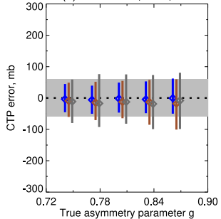
(c) CTP error, OCI, ice
