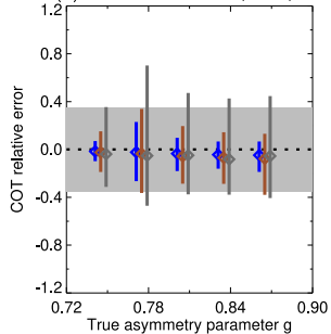
(b) Scaled COT error, OCI, ice
