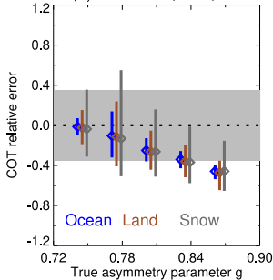
(a) COT error, OCI, ice
