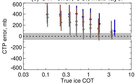
(c) CTP error, OCI, multi-layer
