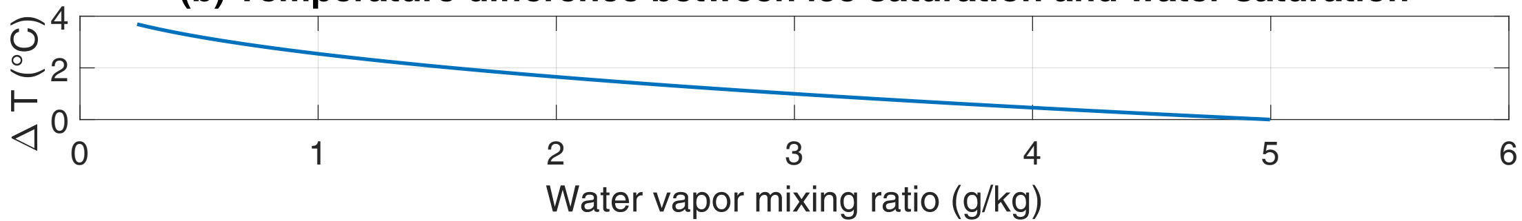
(b) Temperature difference between ice saturation and water saturation
