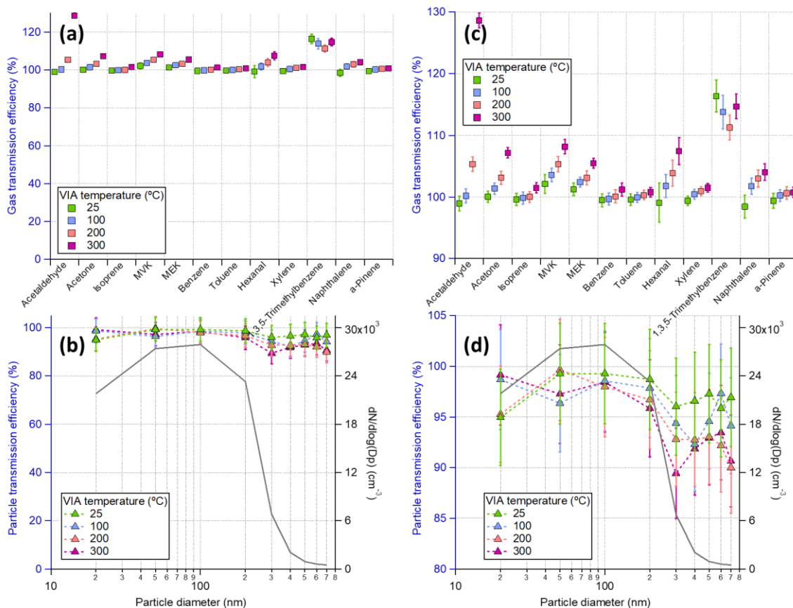
Figure S6. Transmission efficiency of (a) gas compounds (measured by a PTR-TOF) and (b) monodispersed 20-700 nm NaCl particles (measured by a CPC) within the VIA vaporization tube at four different temperatures (25, 100, 200, and 300 °C) with a flow rate of 1 L min -1 . Panels (c) and (d) used the same datasets as panel (a) and (b), respectively, but zoom in to show the details. The reference size distribution of the tested AS particles is shown as grey lines in panel (b) and (d).
