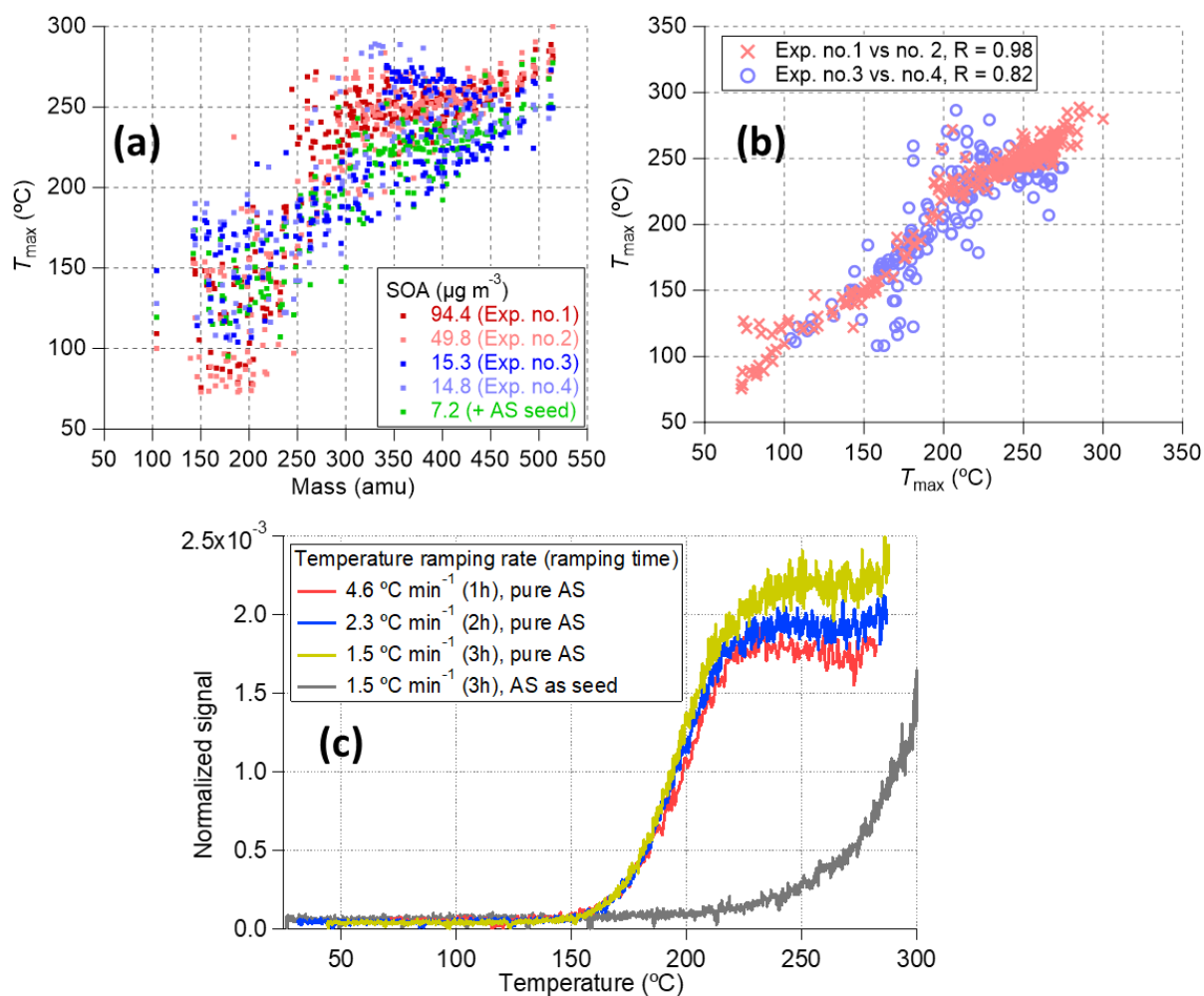
Figure S14. (a) The VIA datasets used to make the mean and the standard deviation of T_{\max} in Figure 7a. (b) Comparisons of T_{\max} obtained from different experiments. (c) Thermogram of sulfuric acid evaporated from 100-nm ammonium sulfate (AS) particles in different experiments.
