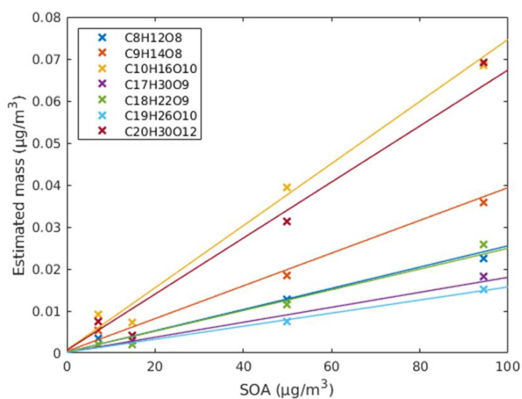
Figure S18. Estimated mass concentrations of HOM species vs. SOA. Some data points were missing because of relatively messy thermograms.
