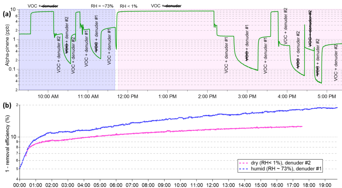
Figure S5. Time series of alpha-pinene during (a) gas denuders test under humid (light blue area) and dry (light red area) conditions and (b) continuous exposure to VOC under dry and humid conditions. In panel (a), the inserted text explains the condition of each stage, i.e. different combinations of VOC flow and gas denuder, and strikethrough means without. The performance of these two gas denuders is summarized in Table S4.
