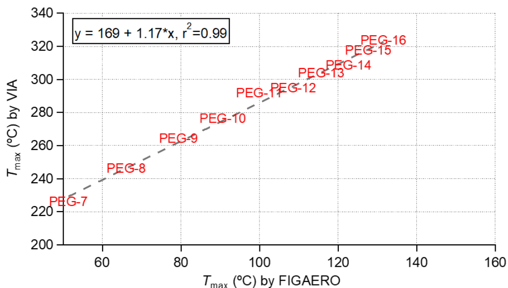
Figure S13. Comparison of T_{\max} measured for the homogenous series of PEGs using the VIA-NO 3 -CIMS and FIGAERO-iodide-CIMS systems. The T_{\max} for PEGs obtained from the VIA-NO 3 -CIMS system are summarized in Table S4.
