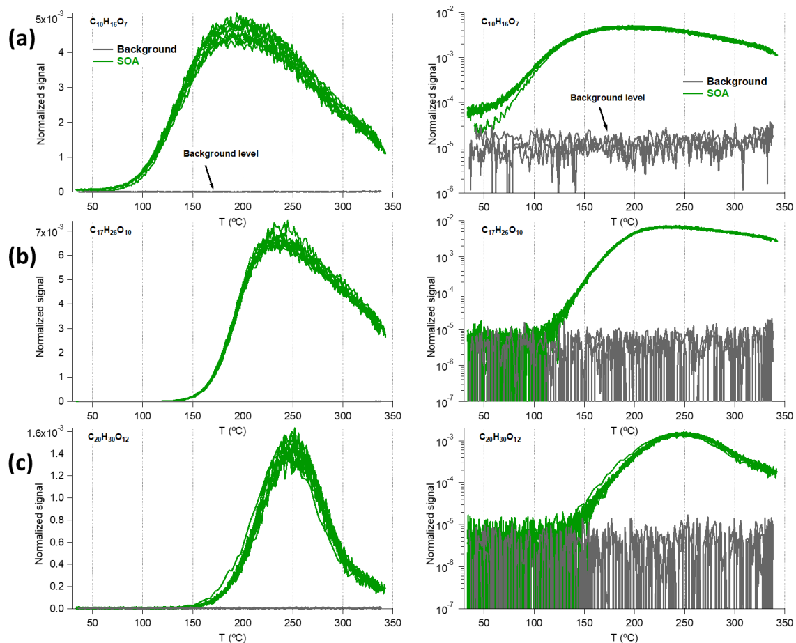
Figure S15. Thermograms during SOA (green lines) and background (gray lines) measurements. The left panels are in linear scale, while the right panels are in log scale. The experiment was conducted in a 2 m 3 Teflon chamber with 90 ppb of \alpha -pinene and 62 ppb O 3 . The three background measurements were conducted before, during, and after the 12 continuous ramping scans.
