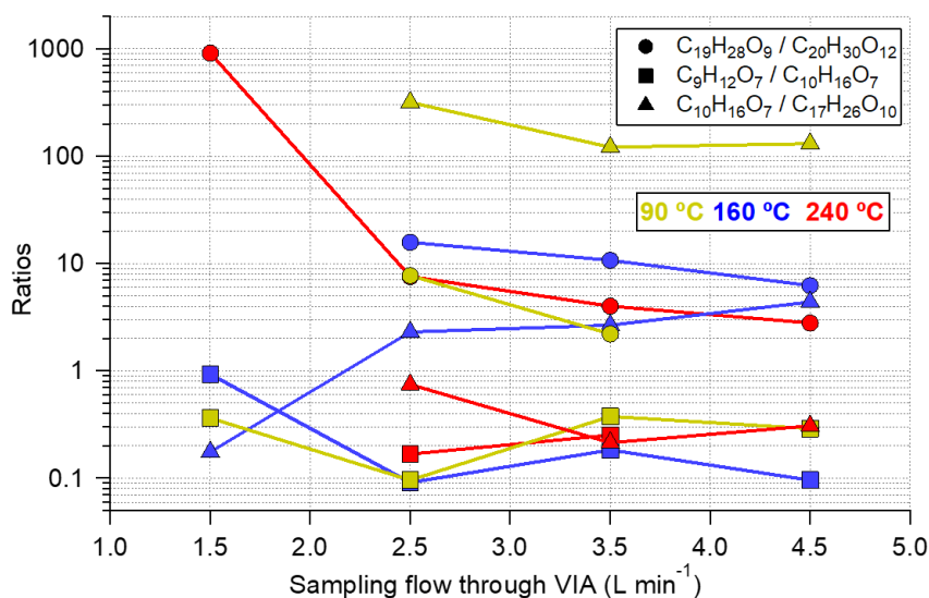
Figure S10. Relative changing between HOM species (circle: two different dimers, square: two different monomers, and triangle: one monomer and one dimer) as a function of sampling flow rate.
