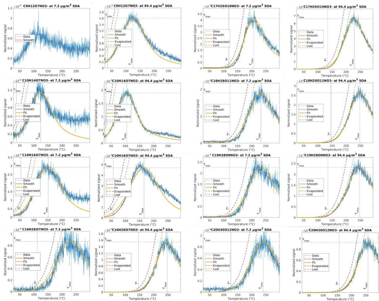
Figure S16. More examples of the fitting results compared to the measured thermograms of different HOM species.
