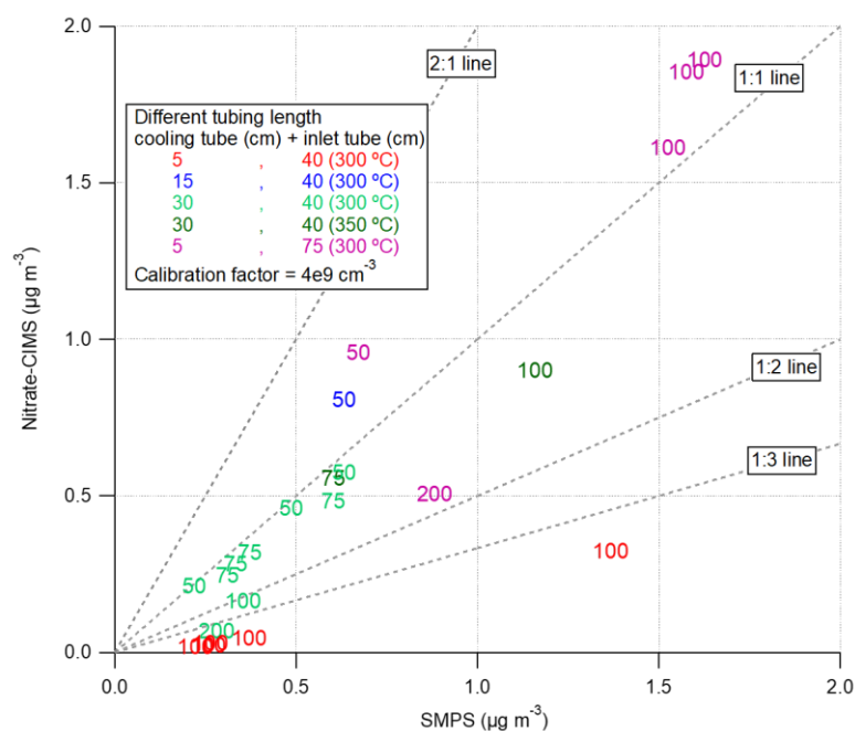
Figure S7. Comparison between the sulfuric acid concentrations measured by the NO 3 -CIMS vs. the evaporated sulfuric acid mass estimated from the SMPS measurements. Different colors represent different setups used for this comparison and the number of each marker shows the size of ammonium sulfate particles (nm) selected.
