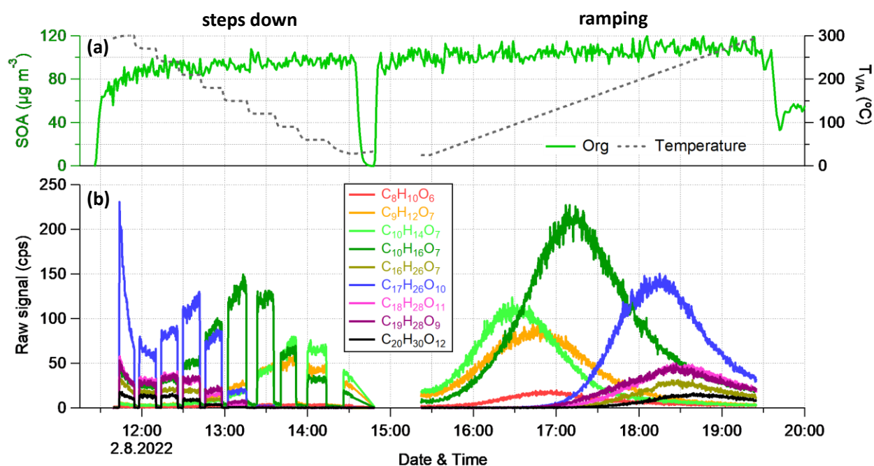
Figure S11. Comparisons between the “steps” and “ramping” modes for (a) SOA measured by the AMS (1.5 min) and temperature of the VIA vaporization tube monitored by a thermocouple, and (b) HOM species (10-s data set). Note that the measurement of steps mode was very unstable during the start of the experiments (VIA heated at 300 °C), which was suspected to be affected by contaminations from the previous experiment.
