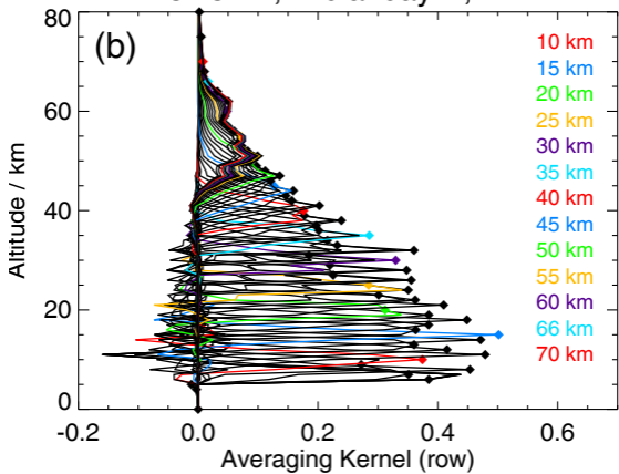
CFC-12, midlat day N, RR
