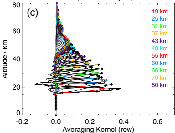
CFC-12, midlat day N, MA
