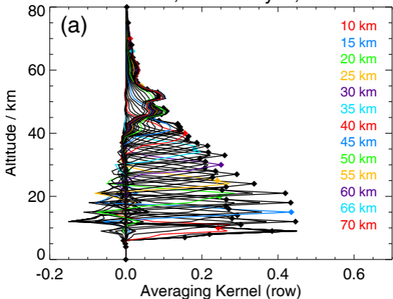
CFC-12, midlat day N, FR
