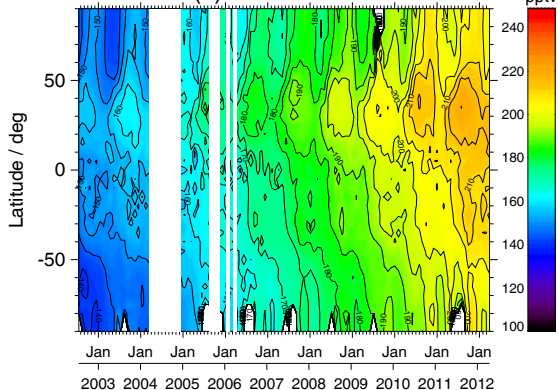
(e) HCFC-22 10 km
