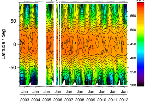
(a) CFC-12 14 km
