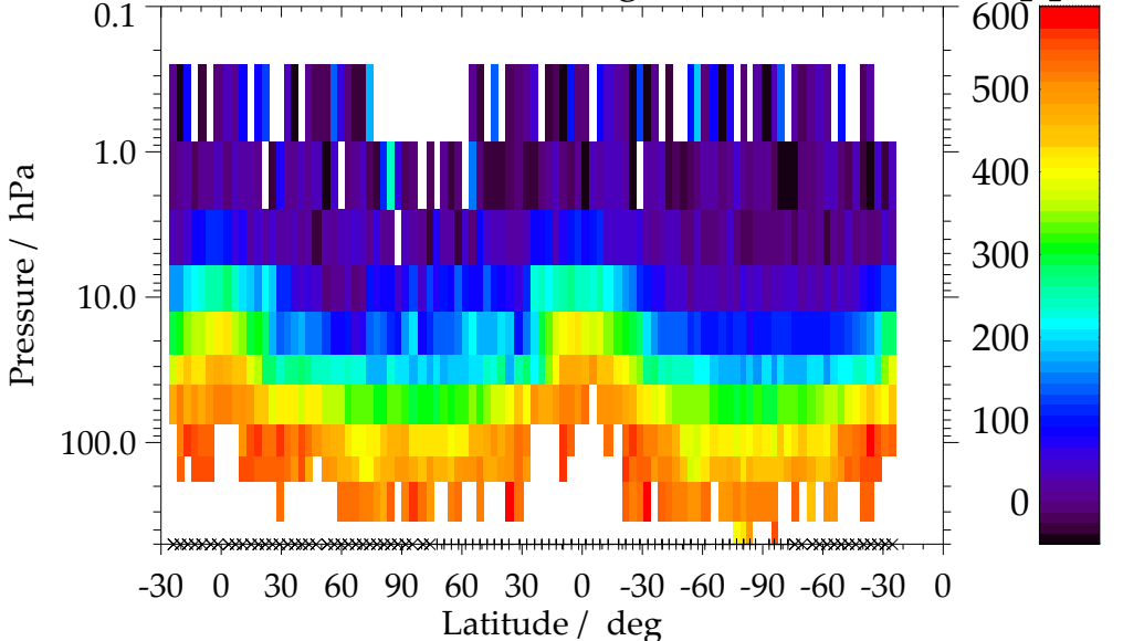
(b) Orbit 36319 coarse grid retrieval
