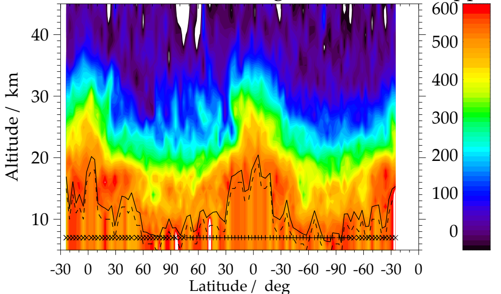
(b) Orbit 36319 coarse grid retrieval
