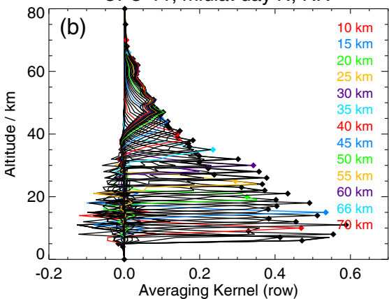
CFC-11, midlat day N, RR
