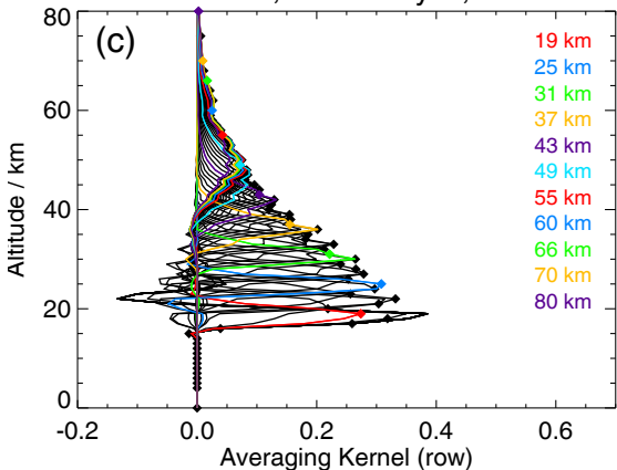
CFC-11, midlat day N, MA
