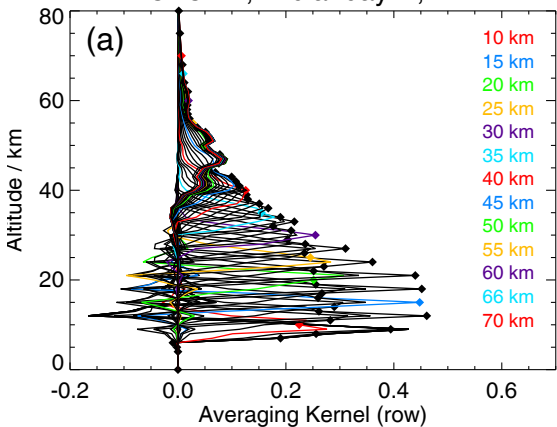
CFC-11, midlat day N, FR
