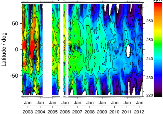
(a) CFC-11 10 km
