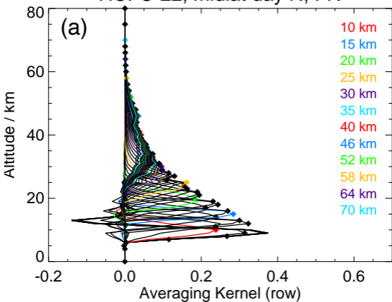
HCFC-22, midlat day N, FR
