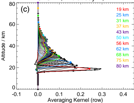
HCFC-22, midlat day N, MA
