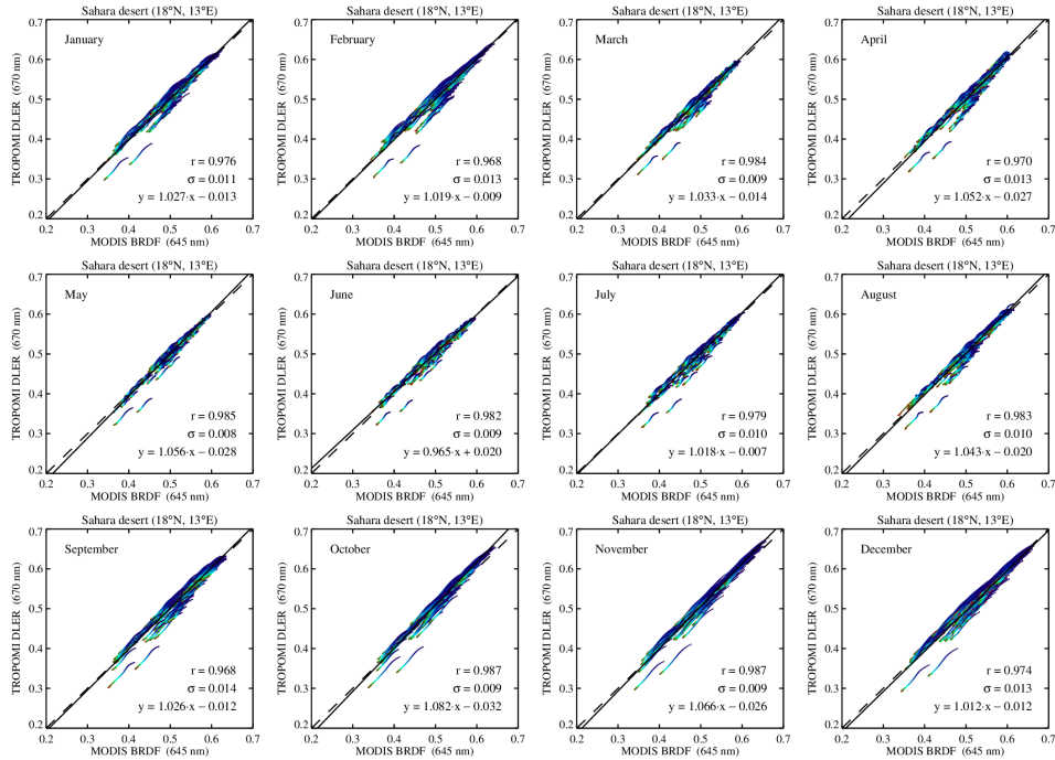
Figure S11. Case 2: TROPOMI surface DLER at 670 nm versus MODIS surface BRDF for the Sahara desert.
