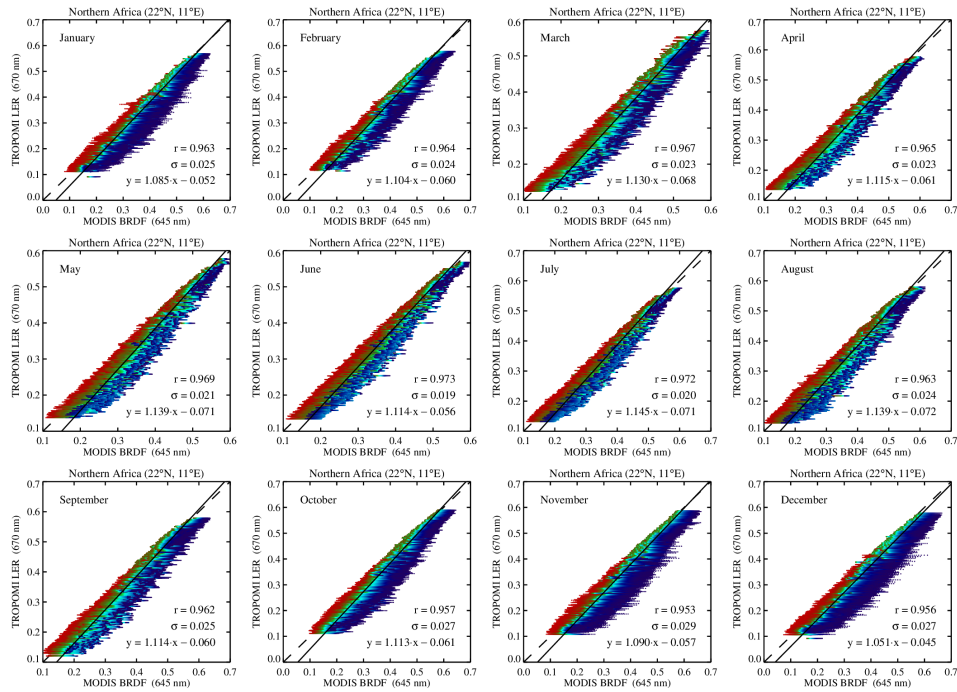
Figure S14. Case 4: TROPOMI surface LER at 670 nm versus MODIS surface BRDF for Northern Africa.
