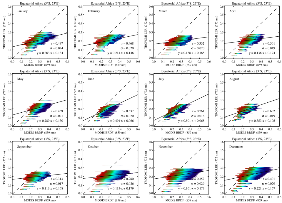
Figure S16. Case 5: TROPOMI surface LER at 772 nm versus MODIS surface BRDF for Equatorial Africa.
