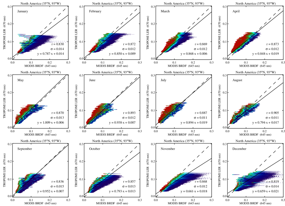
Figure S12. Case 3: TROPOMI surface LER at 670 nm versus MODIS surface BRDF for North America.
