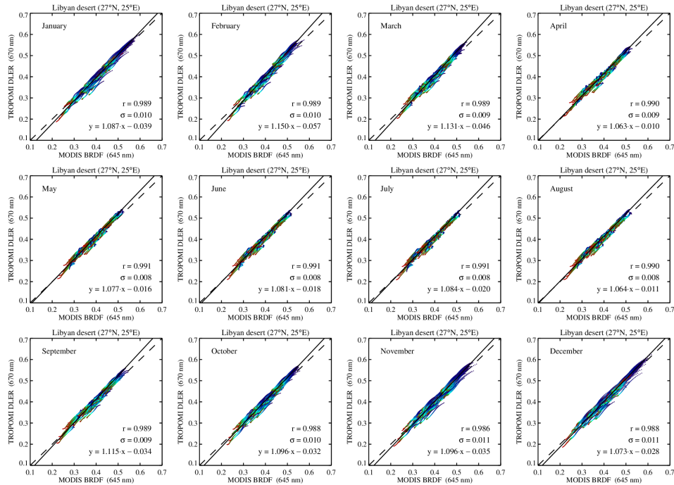
Figure S9. Case 1: TROPOMI surface DLER at 670 nm versus MODIS surface BRDF for the Libyan desert.
