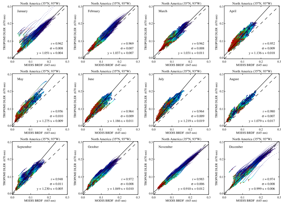
Figure S13. Case 3: TROPOMI surface DLER at 670 nm versus MODIS surface BRDF for North America.
