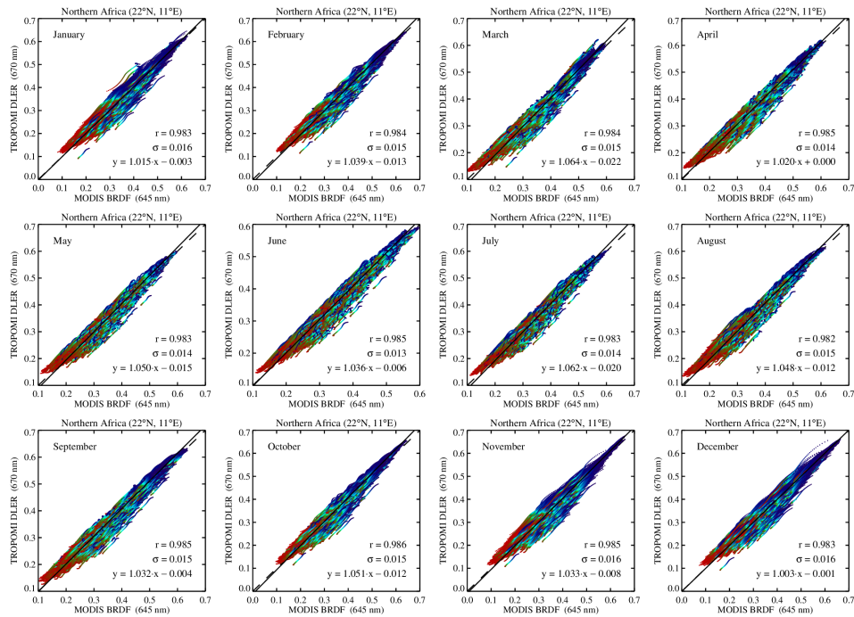
Figure S15. Case 4: TROPOMI surface DLER at 670 nm versus MODIS surface BRDF for Northern Africa.
