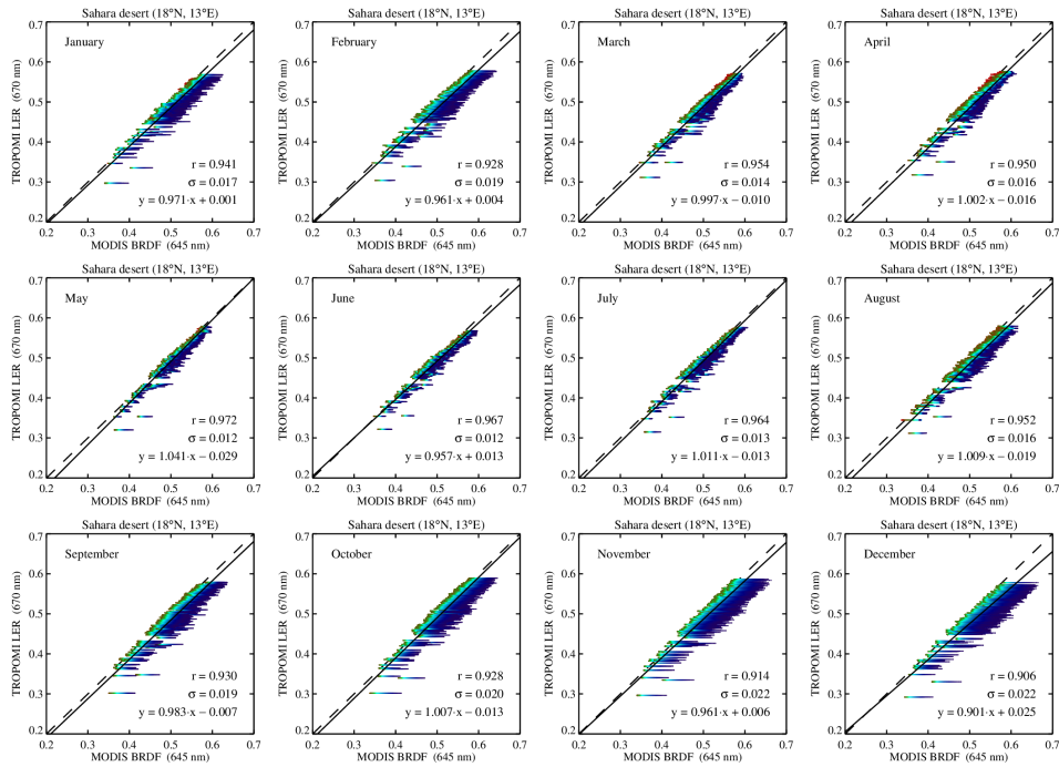
Figure S10. Case 2: TROPOMI surface LER at 670 nm versus MODIS surface BRDF for the Sahara desert.
