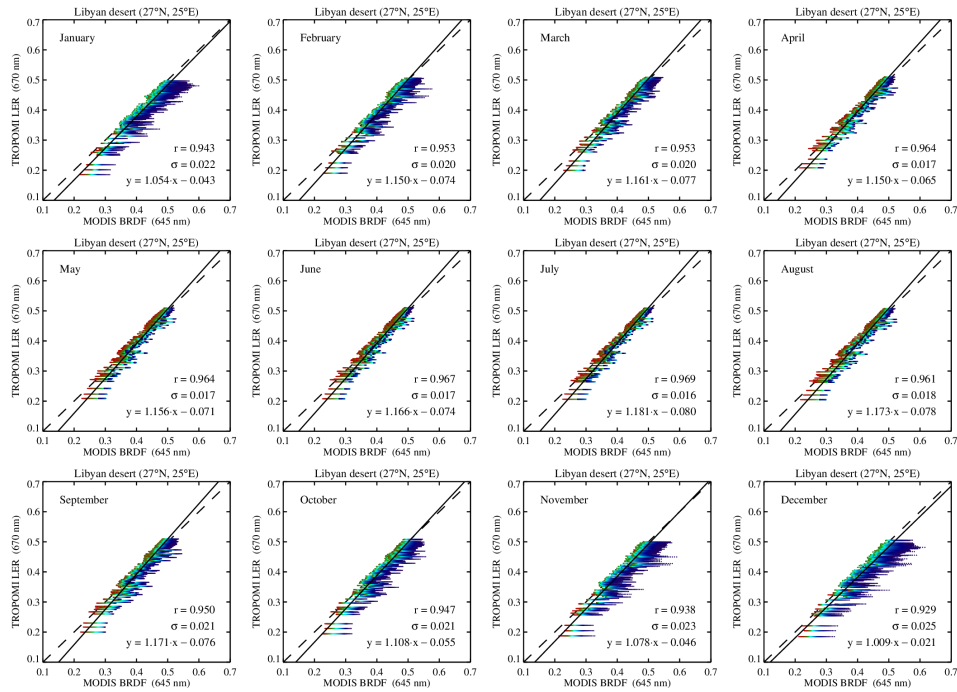
Figure S8. Case 1: TROPOMI surface LER at 670 nm versus MODIS surface BRDF for the Libyan desert.
