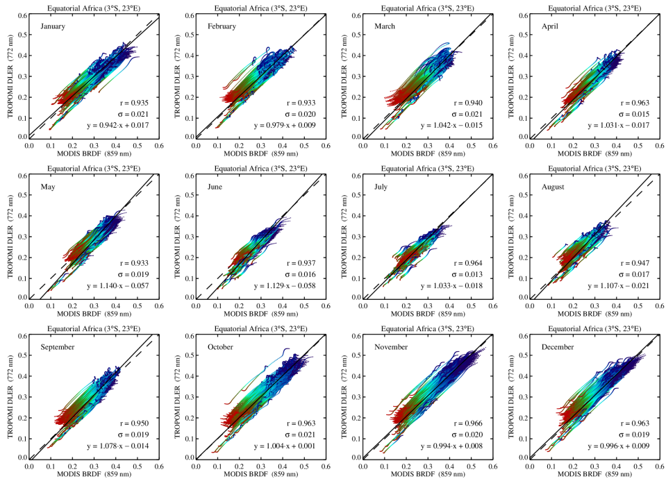
Figure S17. Case 5: TROPOMI surface DLER at 772 nm versus MODIS surface BRDF for Equatorial Africa.
