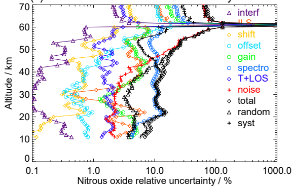
(c) Northern midlatitude summer day FR
