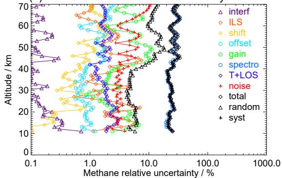
(a) Northern midlatitude summer day FR
