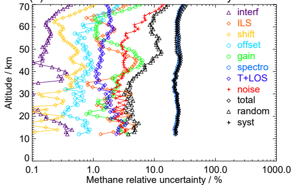
(b) Northern midlatitude summer day RR
