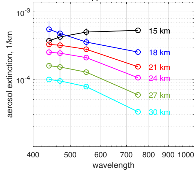
(f) AERGOM
