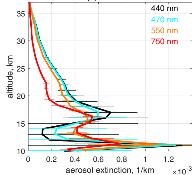
(f) AERGOM
