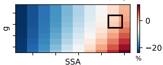
(e) Mean bias in Xalb , \Delta XCH_4 -only
