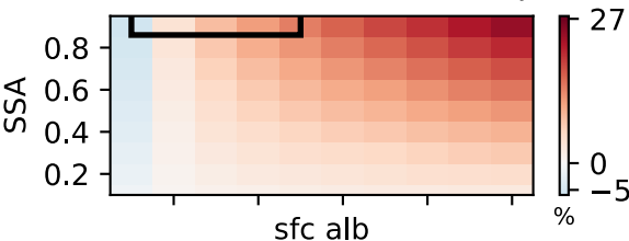
(c) Mean bias in \Delta XCH_4 , \Delta XCH_4 -only
