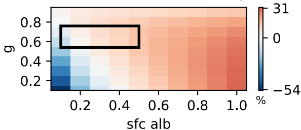
(c) Mean bias in \Delta XCH_4 , \Delta XCH_4 -only
