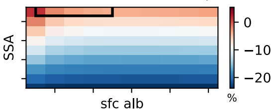
(f) Mean bias in Xalb , \Delta XCH_4 -only
