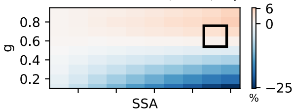
(b) Mean bias in \Delta XCH_4 , \Delta XCH_4 -only
