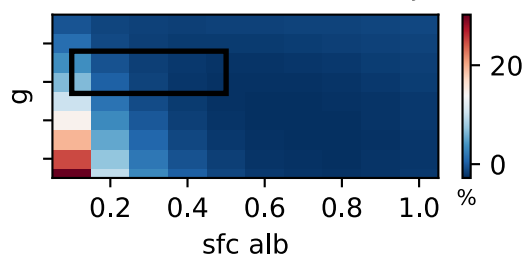
(f) Mean bias in Xalb , \Delta XCH_4 -only
