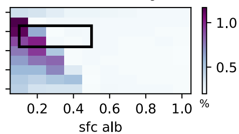
(f) SD in X_{alb} , multi-angle
