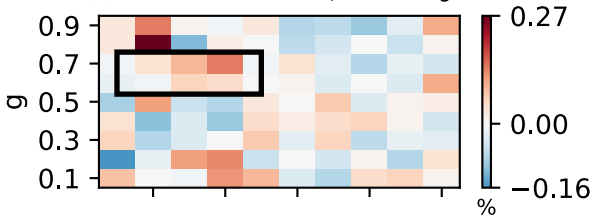
(b) Mean bias in AOD, multi-angle
