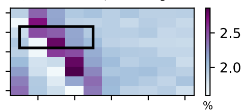
(e) SD in AOD, multi-angle
