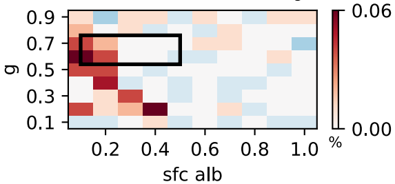
(c) Mean bias in X_{alb} , multi-angle
