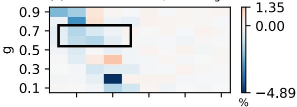
(c) Mean bias in X_{alb} , multi-angle
