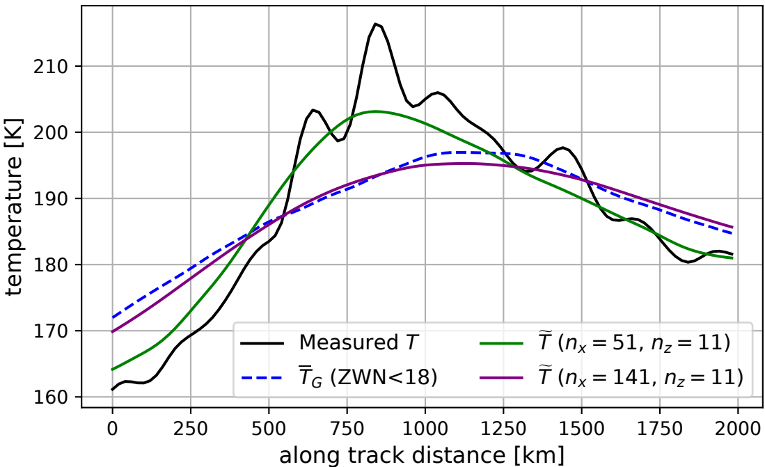
Polynomial smoothing of the temperature field at 80 km
