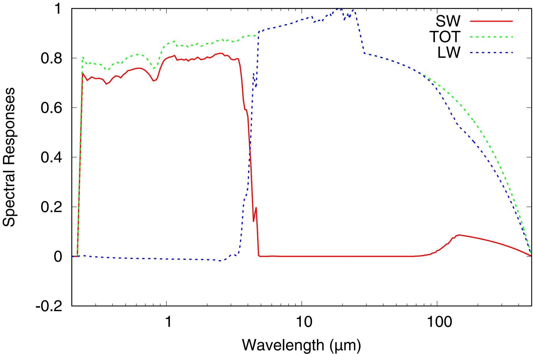
EarthCARE BBR Spectral Responses Nadir (Model CCDB May 2019)
