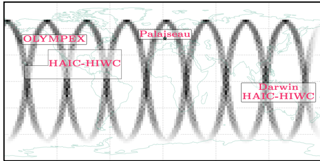
(b) GridSat
