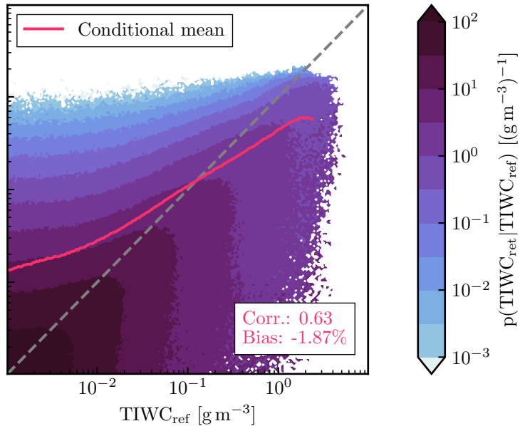
(b) GridSat
