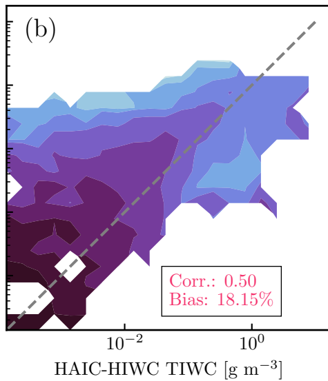
GridSat
