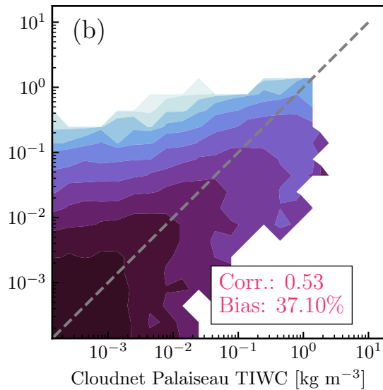
GridSat
